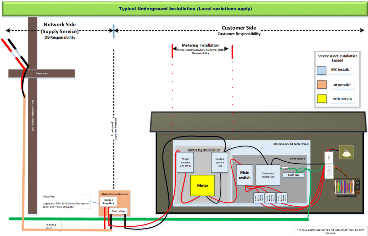
Figure 1 Typical Underground Installation
